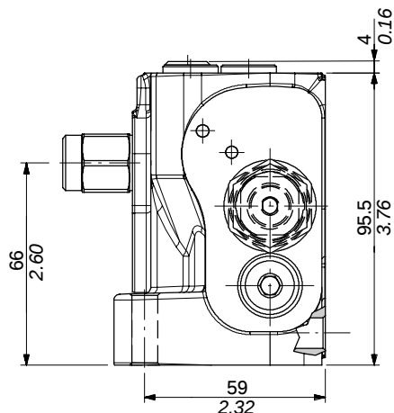
Pressure reducing valve VRPF Wrench 19 - 42 Nm / 31 lbft
