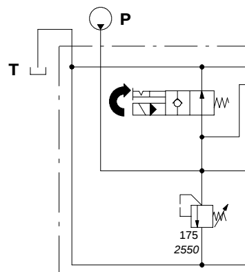
Description example: CN(TVG3-175)ELT-12VDC-SAE
