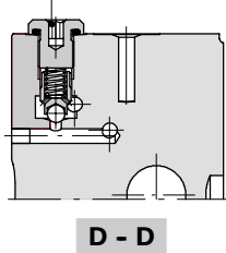
Relief valve VLP Allen wrench 4 6.6 Nm / 4.9 lbft
