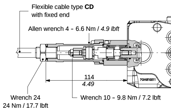
Positioner type 8TL with kit TQ50
