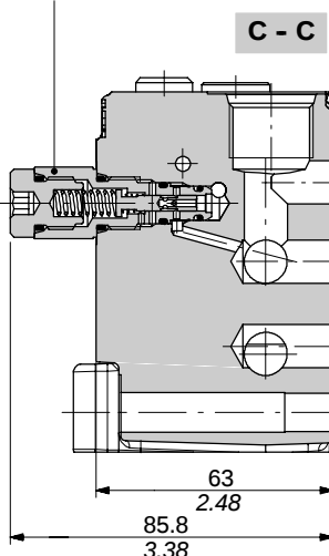
Pressure reducing valve VRPF Wrench 19 - 42 Nm / 31 lbft
