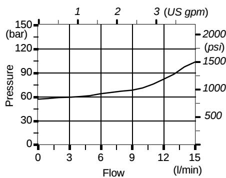
VLP relief valve performance curve
