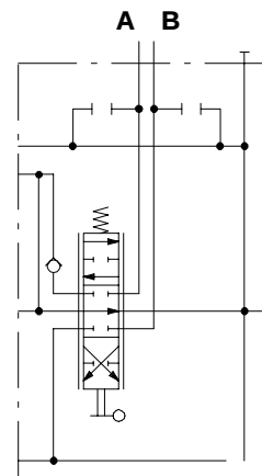
Description example: RPS-101-8L.UTUT-F-SAE
