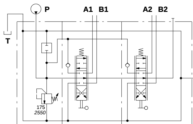
Closed center circuit
