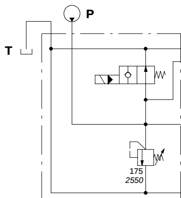
Description example: CN(TVG3-175)ELN-12VDC-SAE
