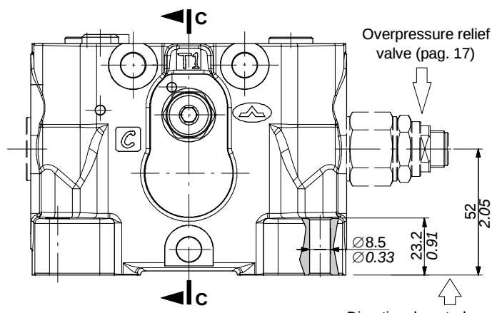
Overpressure relief valve (pag. 17) Directional control valve mounting face
