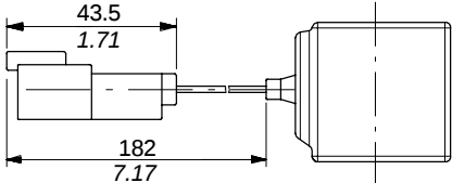
Coil with Deutsch DT connector
