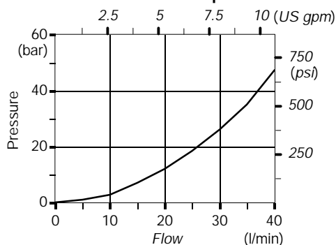
Pressure drop
