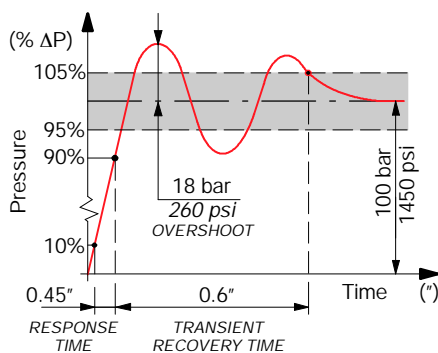
Response time
