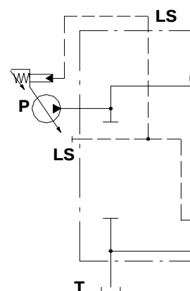
Hydraulic circuit
