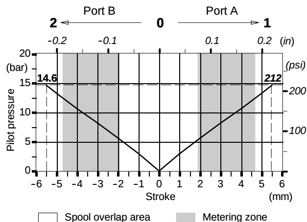
Pilot pressure - stroke diagram
