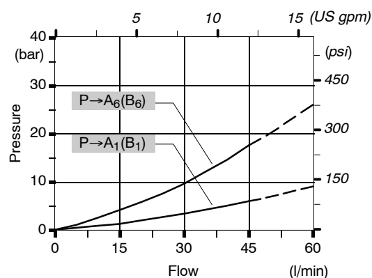
Pressure drop P→A(B)
