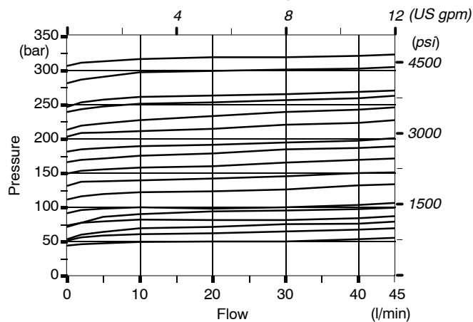
Pressure-flow diagram
