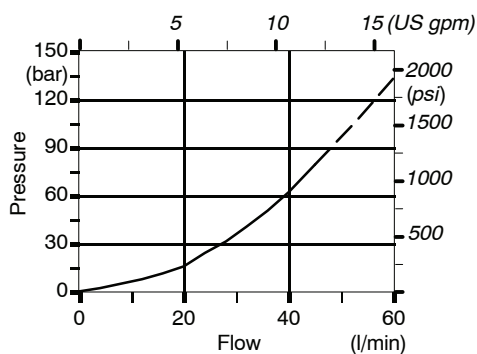
Pressure drops
