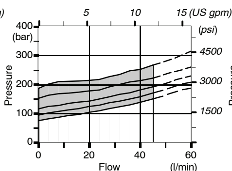
Pressure drops
