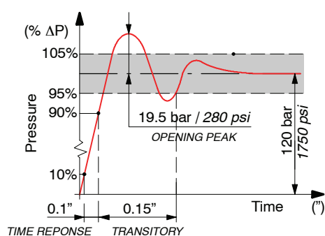
Time response
