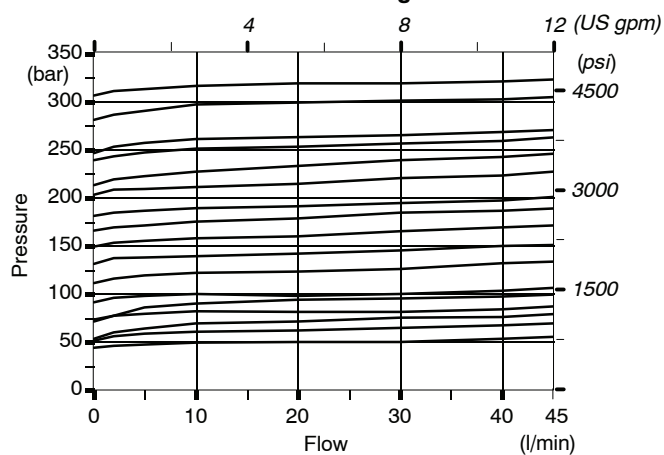
Pressure-flow diagram
