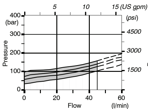
Pressure drops
