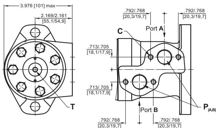
Side Ports
