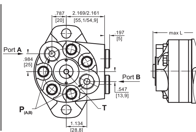
Rear Ports
