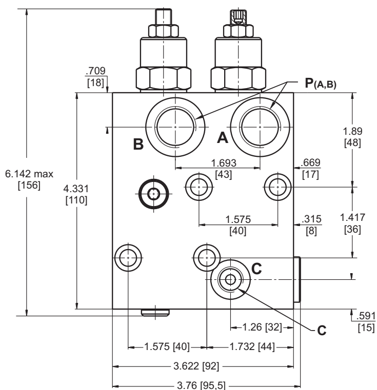
DUAL VALVE KPBR-250/1/D...
