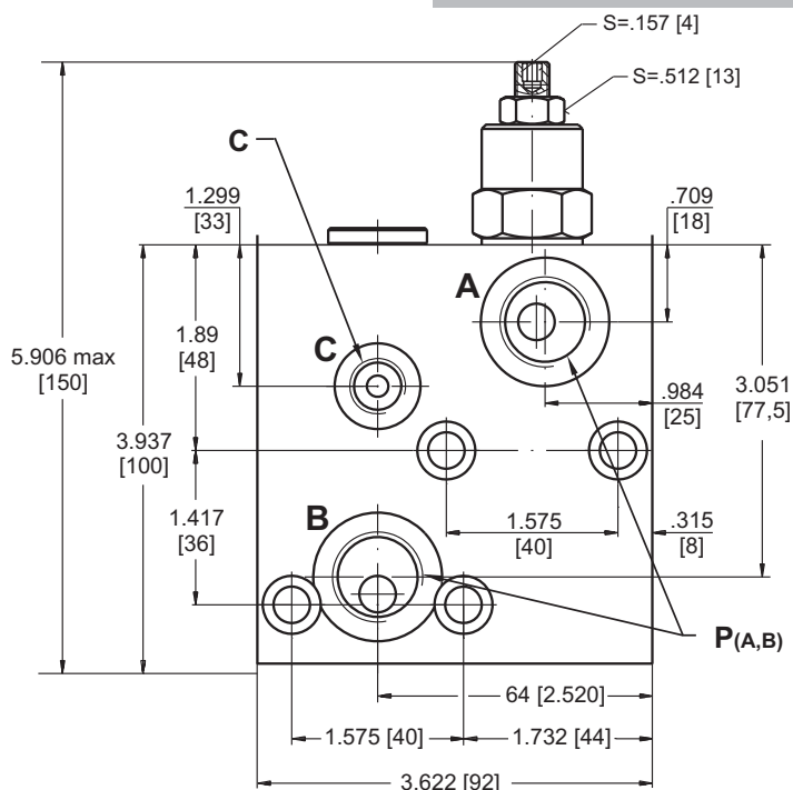
SINGLE VALVE KPBR-250/1/E...
