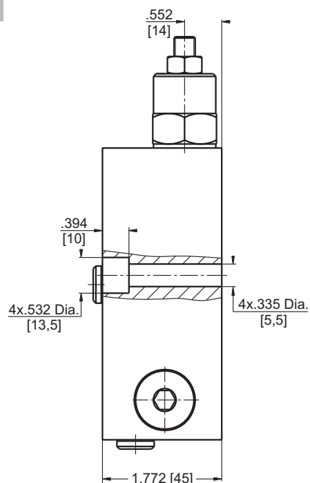
DUAL VALVE KPBR-250/1/D...
