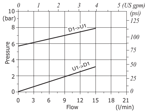
VBPDL 14/SO pressure drop vs. flow
