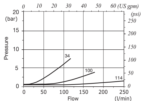
VUC/M34-100-114 pressure drop vs. flow opening pressure 0.5 bar (7.25 psi)
