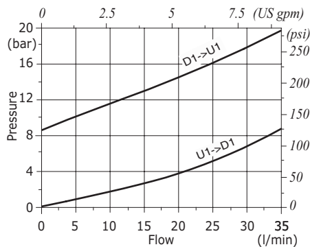
VBPDL 38/SO pressure drop vs. flow
