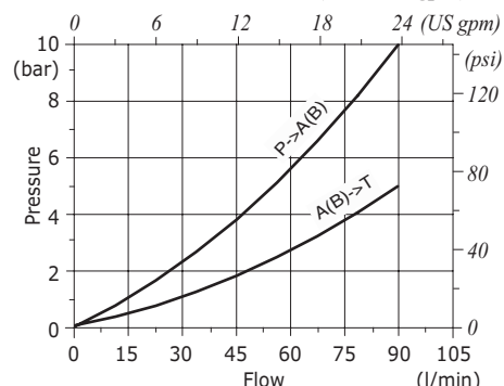
SD11/IAM 12 pressure drop vs. flow
