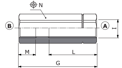
Housing type VDR/CO/F
