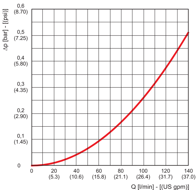
HF 650-30 (G 1)
