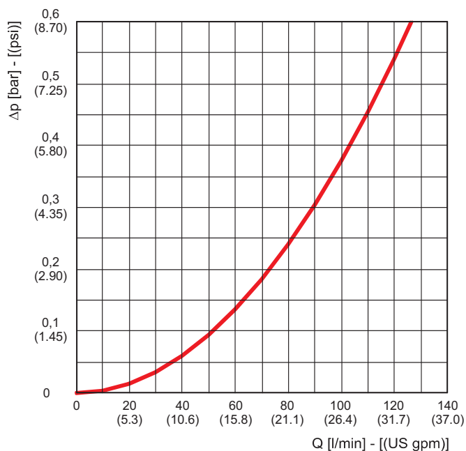
HF 650-20 (G3/4)
