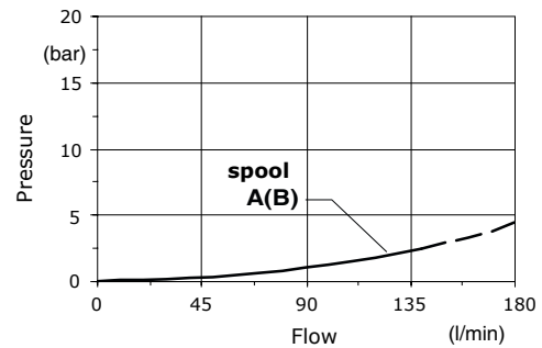
Pressure drop versus flow A → C(E)
